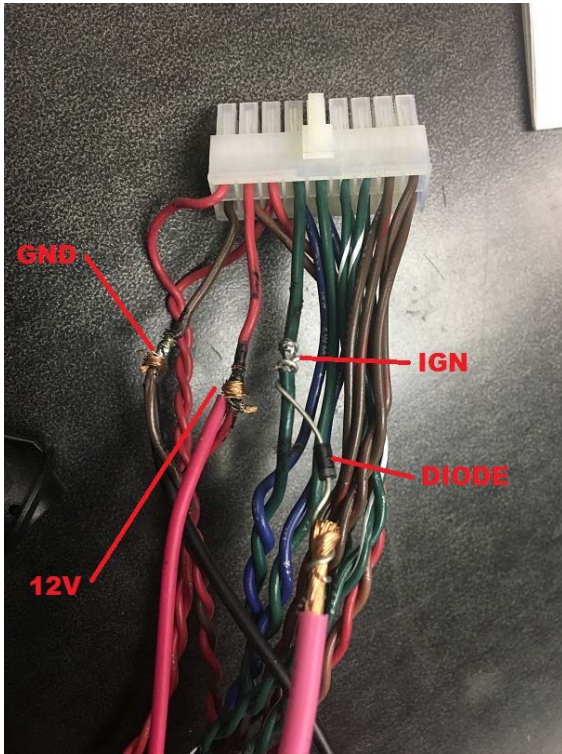
Directed Remote Start Connection
