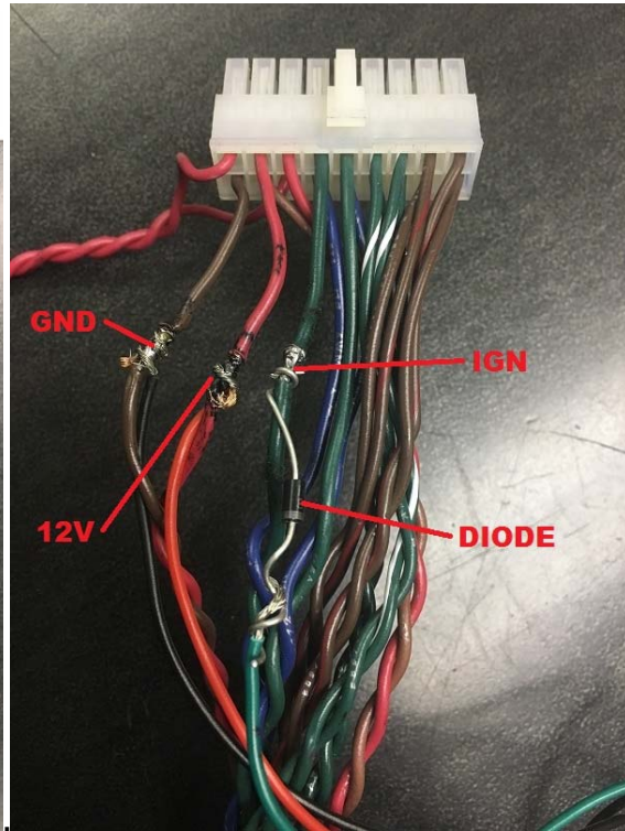
Compustar Remote Start Connection
