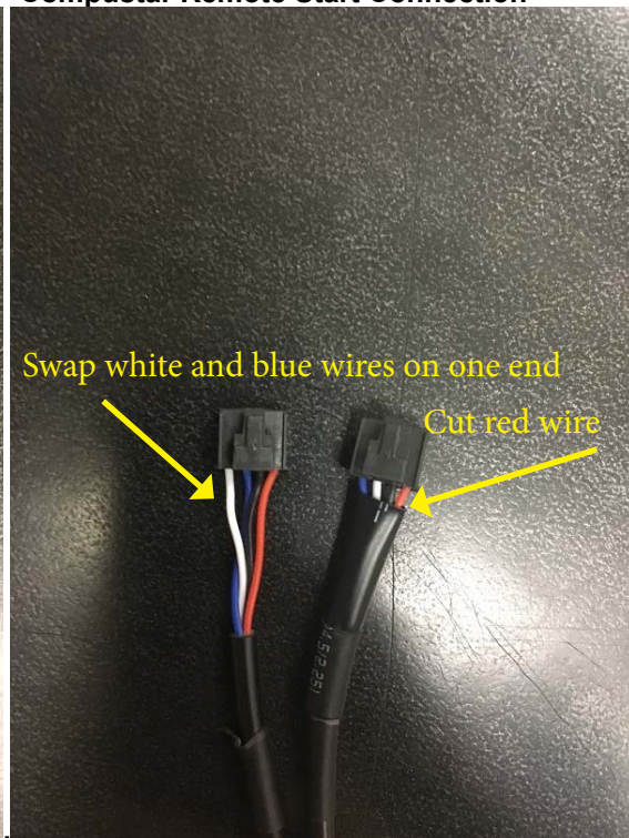
Compustar Data Cable (pin 1,2 are crossed)
